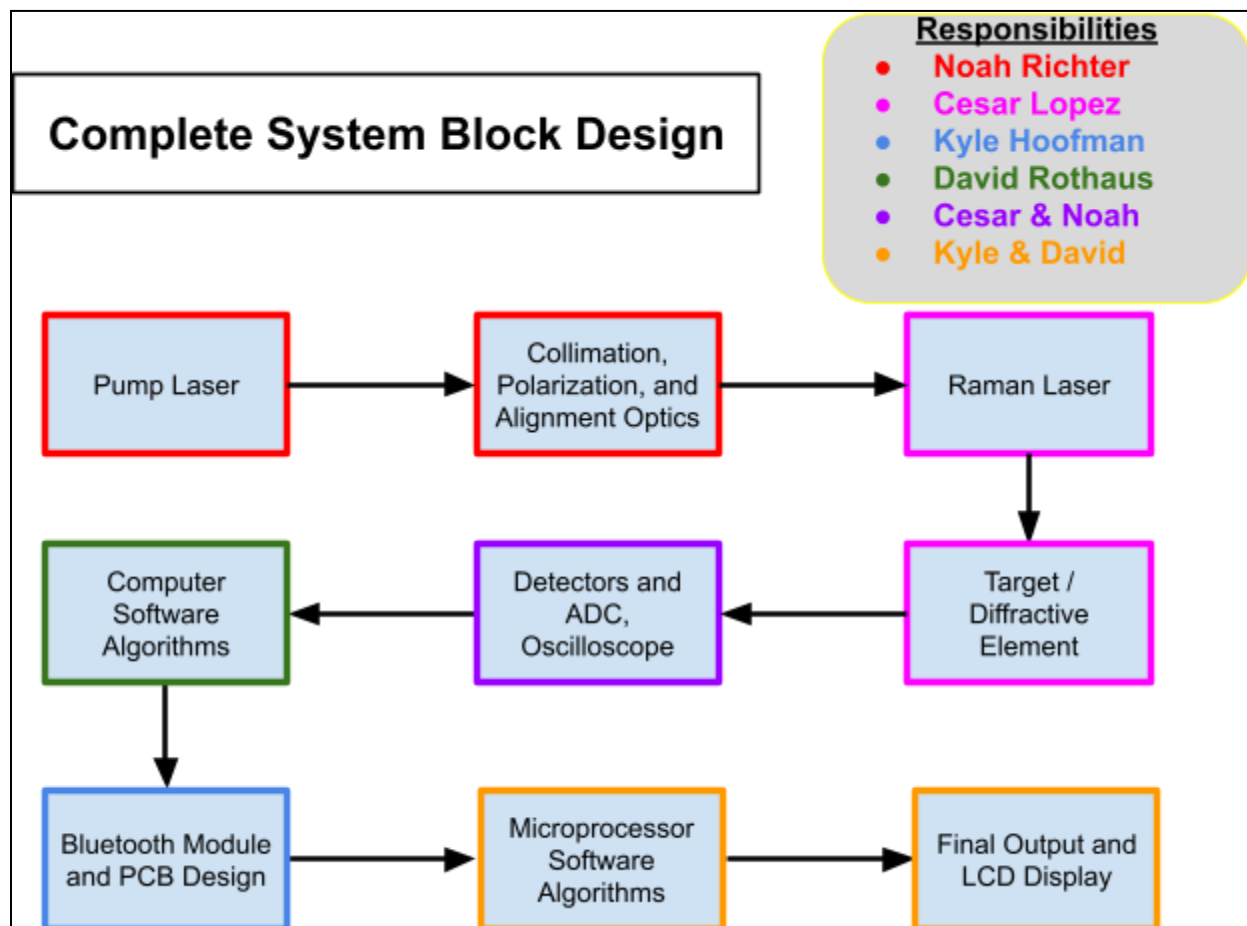
Fig. 2: Complete System Block Diagram
