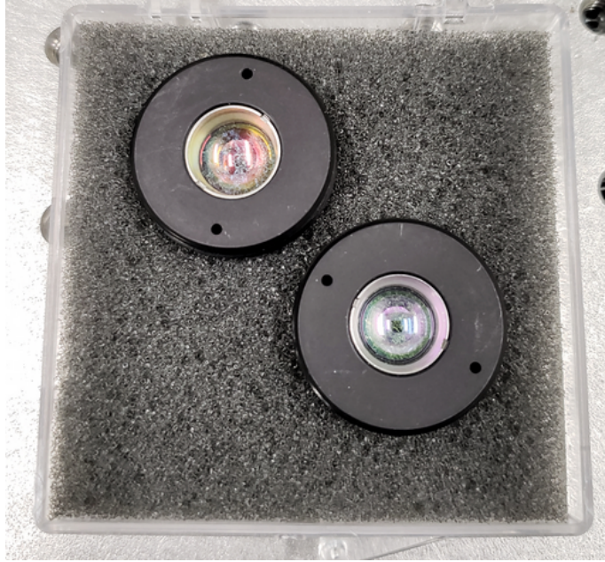
Fig. 68: Pair of Thorlabs A240TM-C lenses without any visible laser damage that would impact their performance.
