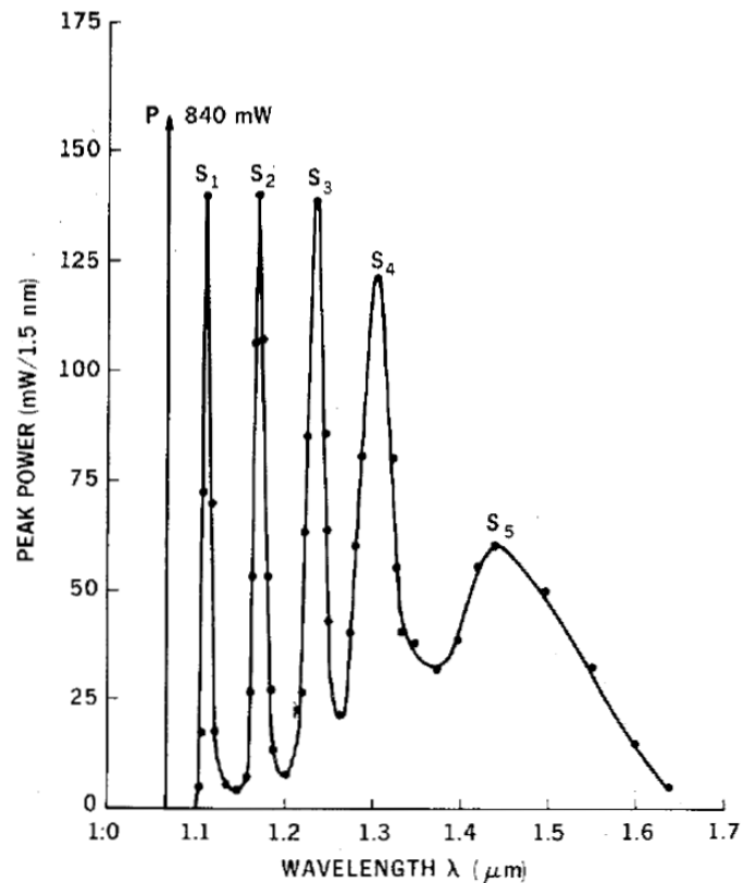
Fig. 13: Emission data of a multispectral single-mode silica fiber Raman laser.
