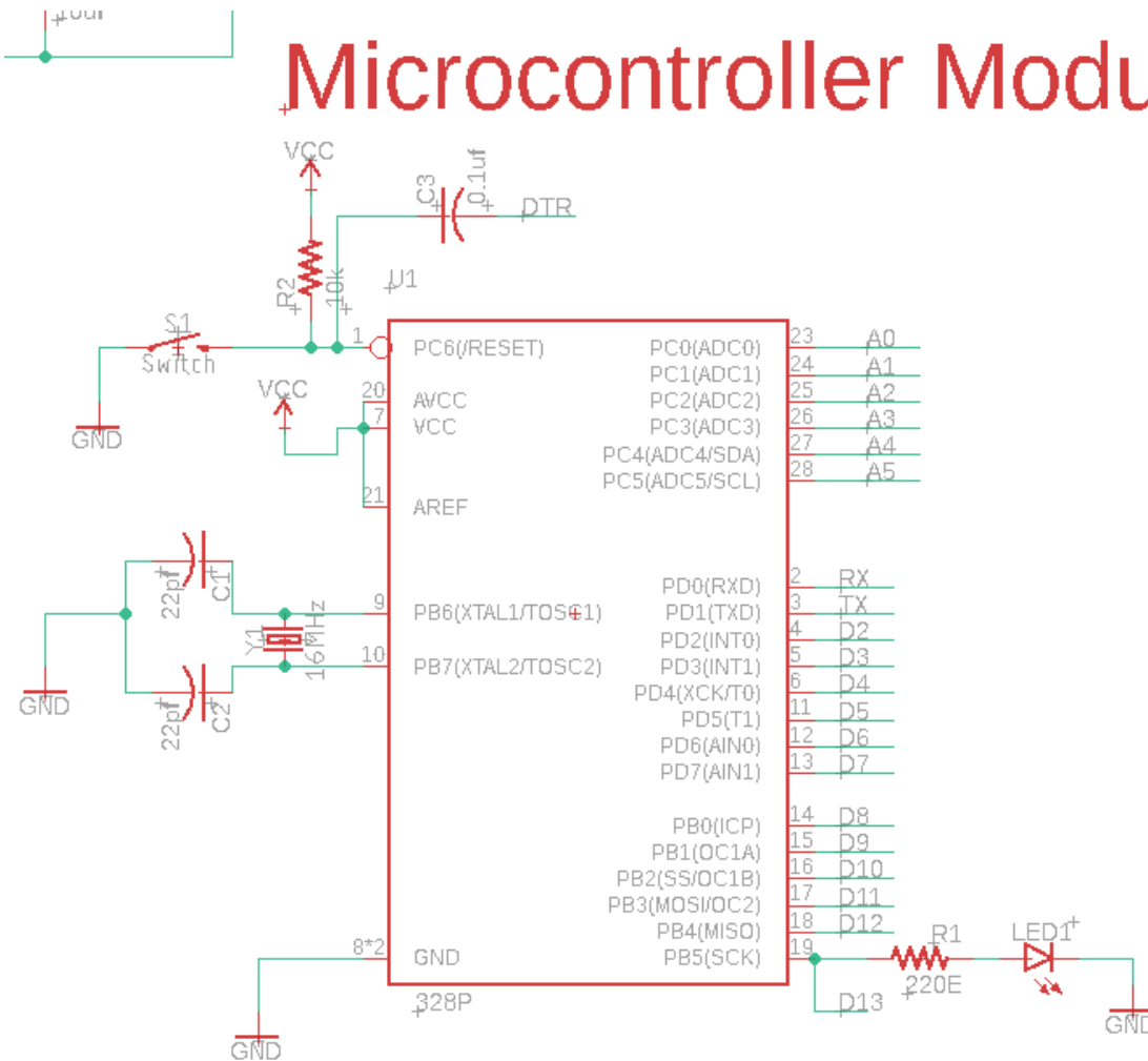
Fig. 50: Schematic of the Microcontroller Module
