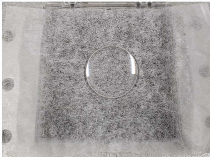
Fig. 67: Newport KBX061 bi-convex uncoated lens for collimating the Raman output. No laser induced damage on its surface and good transmission up to 2000nm wavelength.
