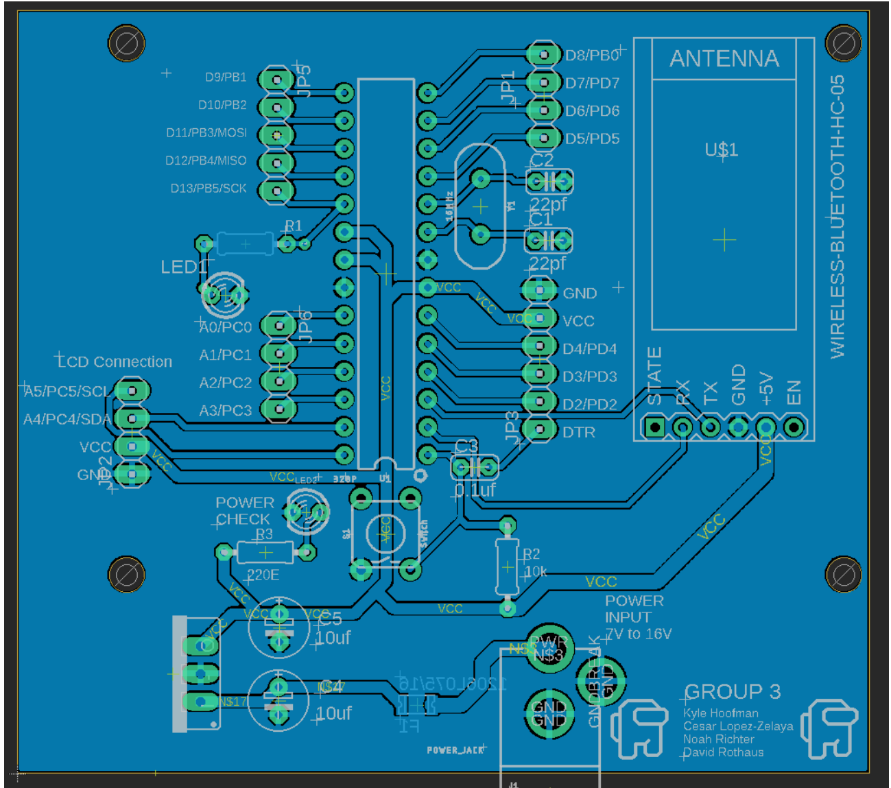
Fig. 63: Custom Microcontroller PCB featuring a ATmega328p-pu that will be connected to and control the external modules
