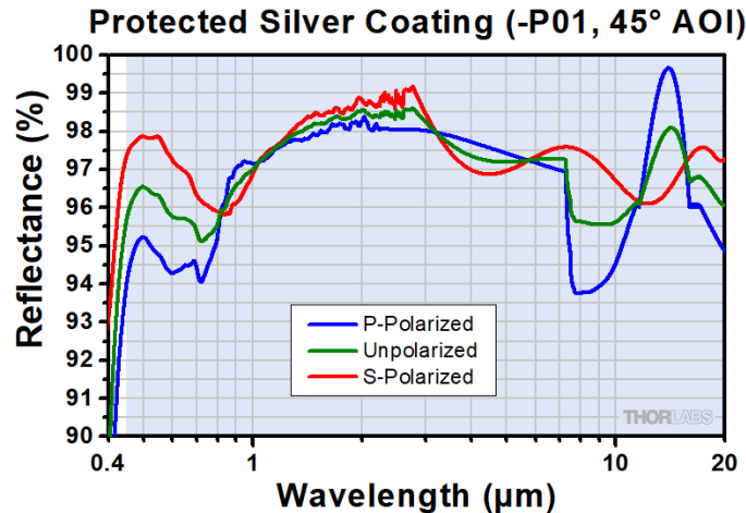
Fig. 36: Conventional Thorlabs silver mirror reflectivity values are two different polarization states and unpolarized light. Excellent reflectivities in the NIR-SWIR reduce the system losses.
